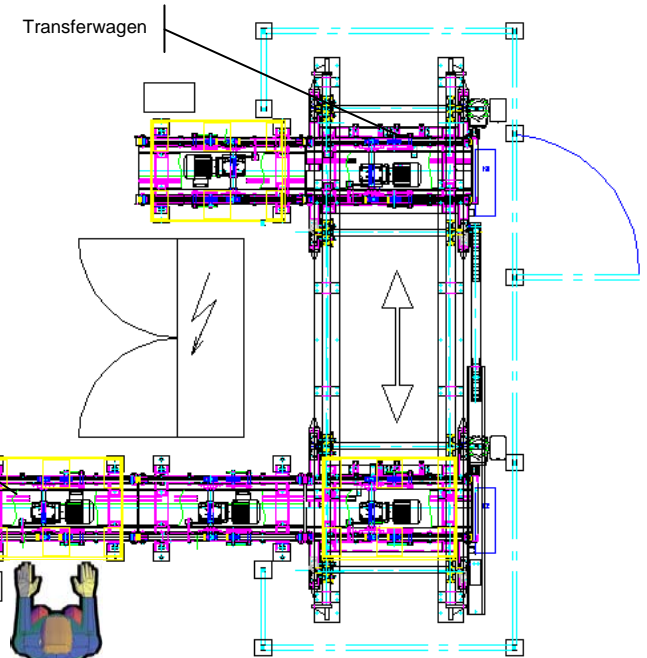
Transferwagen
